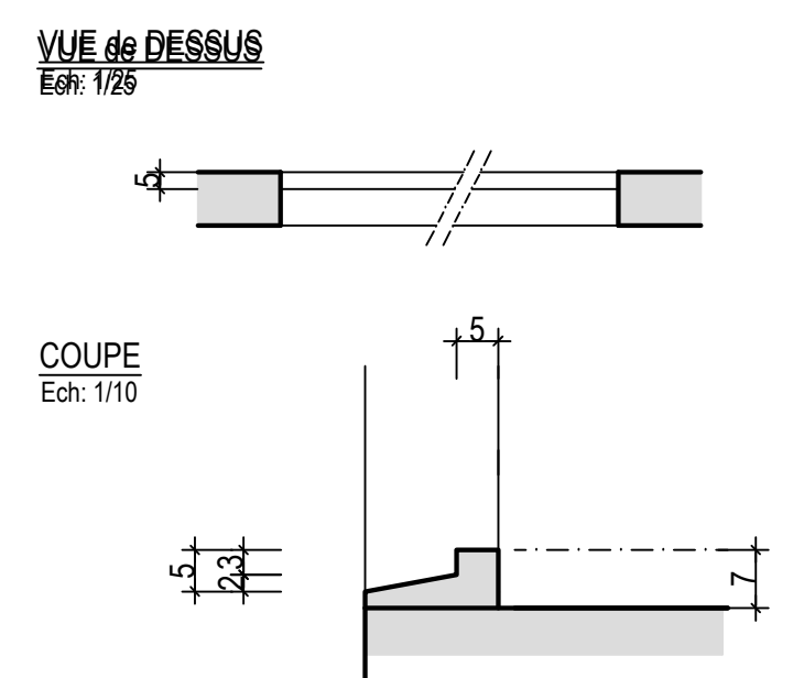
DETAIL "2"
