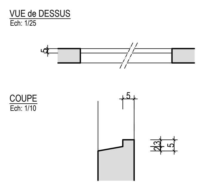
DETAIL "3"
