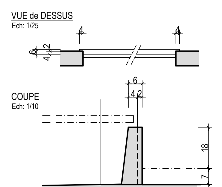
DETAIL "5"
